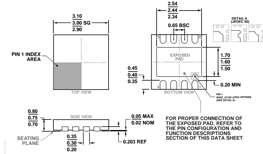
Figure 76. 8-Lead Lead Frame Chip Scale Package [LFCSP] 3 mm x 3 mm Body and 0.75 mm Package Height (CP-8-19) Dimensions shown in millimeters
