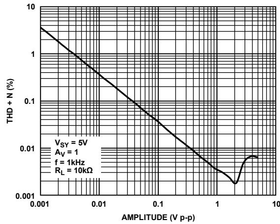
Figure 60. THD + N vs. Amplitude
