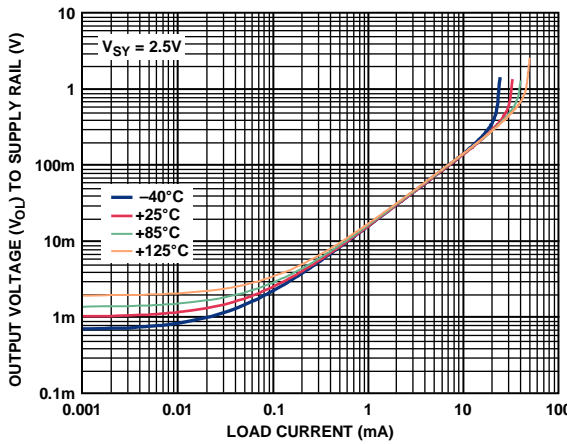
Figure 16. Output Voltage ( V_{O1} ) to Supply Rail vs. Load Current
