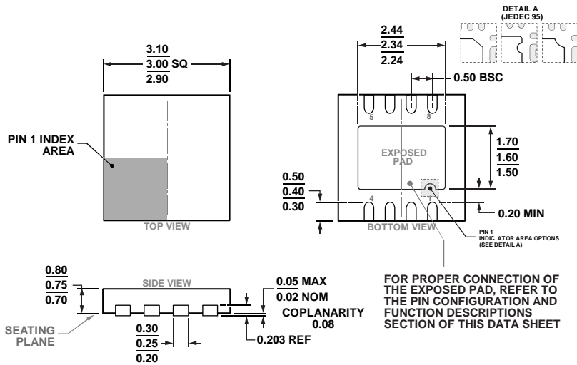
Figure 75. 8-Lead Lead Frame Chip Scale Package [LFCSOP] 3 mm x 3 mm Body and 0.75 mm Package Height (CP-8-11)
