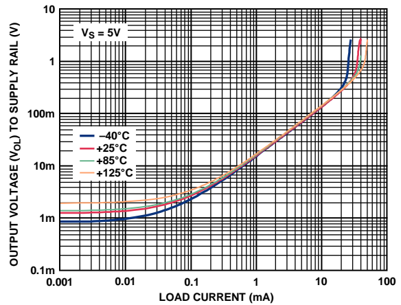
Figure 19. Output Voltage ( V_{O1} ) to Supply Rail vs. Load Current
