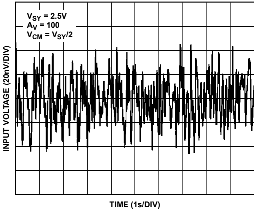
Figure 56. 0.1 Hz to 10 Hz Noise
