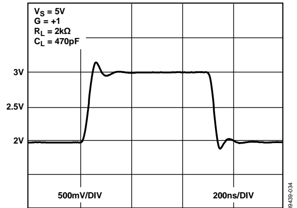
Figure 36. Pulse Response, +V_S = +5V , G = +1 , C_L = 470pF
