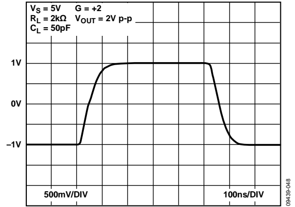
Figure 34. Pulse Response, +V_S = \pm 2.5V , G = +2
