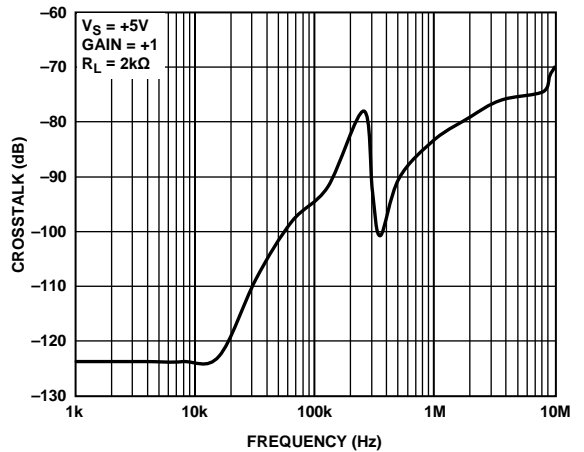
Figure 29. Crosstalk vs. Frequency
