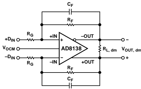
Figure 42. Circuit Definitions
