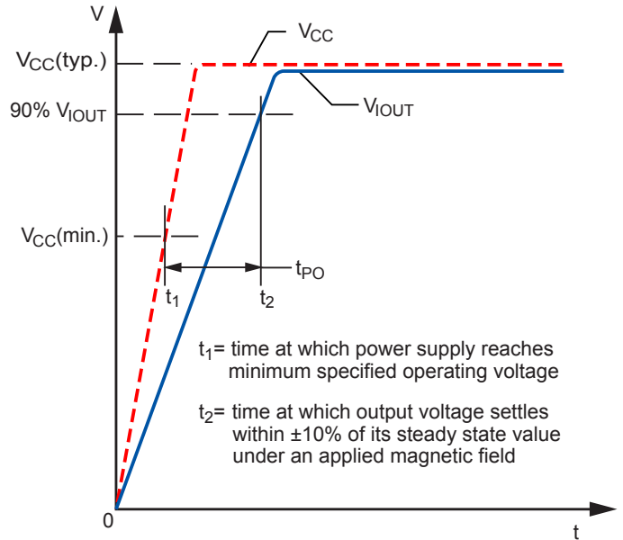
Figure 13: Power-On Time ( t_{PO} )
