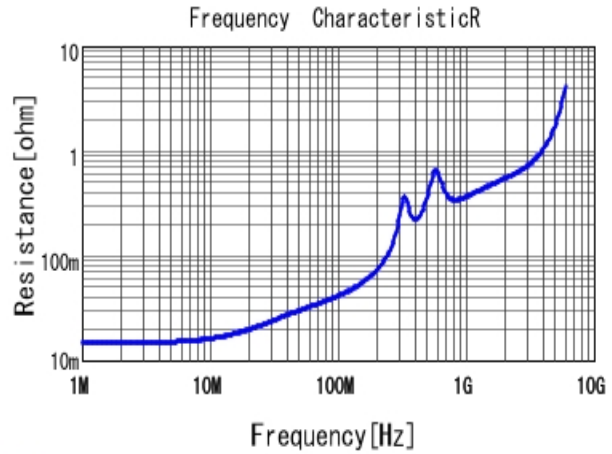
■ GRM3195C2A222JA01 R DCOV, 25degC
