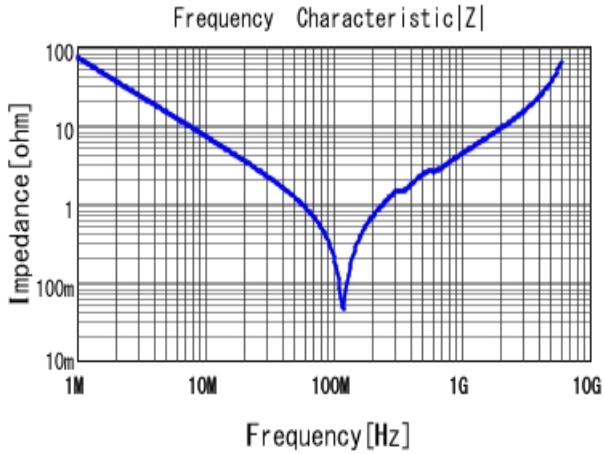
■ GRM3195C2A222JA01 |Z| DCOV, 25degC
