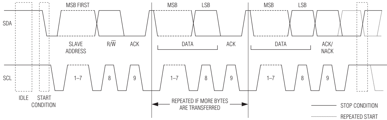
Figure 7. I 2 C Protocol Overview
