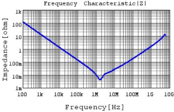
GRT21BR61A226ME13 |Z| DCOV, 25degC
