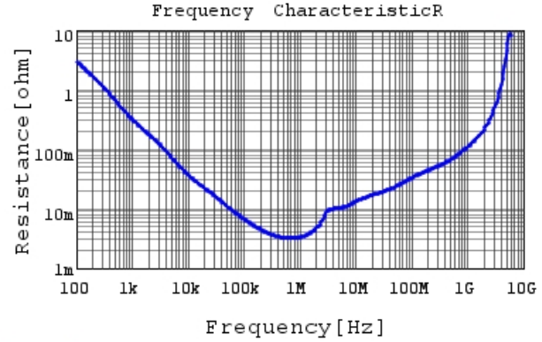
GRT21BR61A226ME13 R DCOV, 25degC
