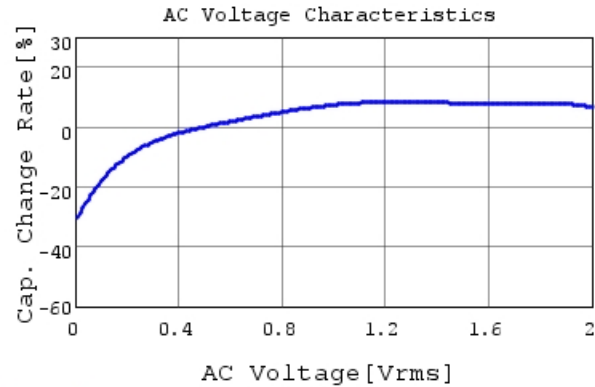
GRT21BR61A226ME13 C-AC Voltage capchange, Dc
