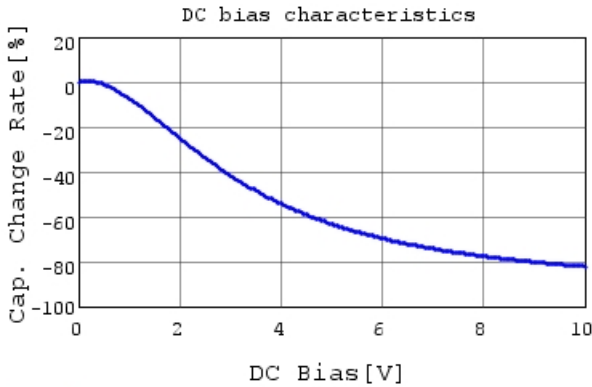
GRT21BR61A226ME13 C-DC bias capchange, 25.0c
