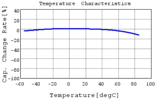
GRT21BR61A226ME13 C-Temp. capchange, DC0.0V,
