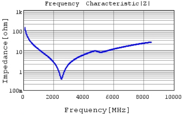
GRM1555C1H120GA01 |Z| DCOV, 25degC
