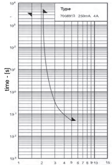
Time-Current Characteristics
