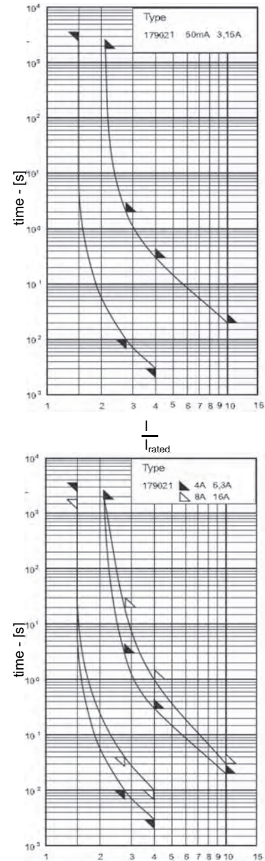
Time-Current Characteristics
