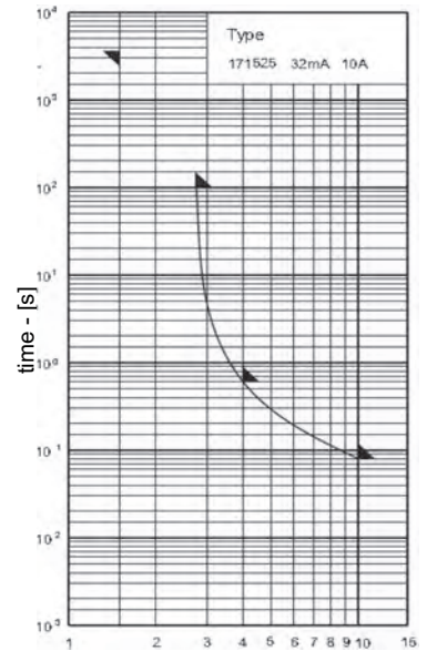
Time-Current Characteristics
