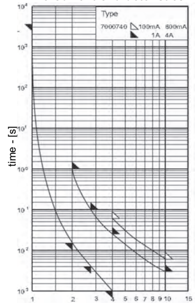
Time-Current Characteristics
