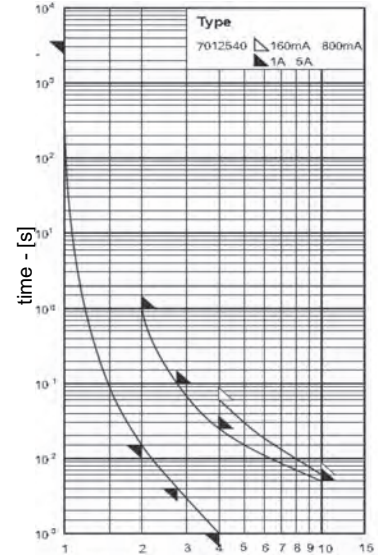
Time-Current Characteristics
