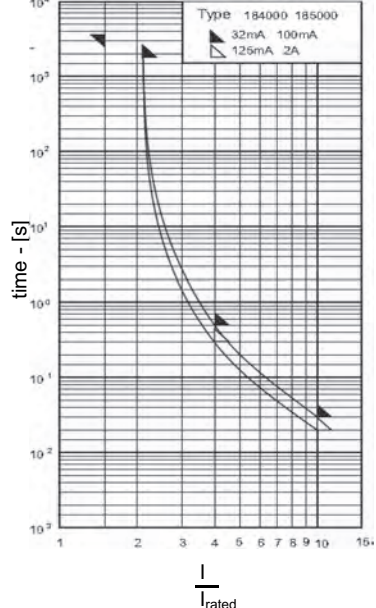
Time-Current Characteristics
