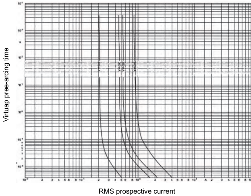
Time-Current Characteristics
