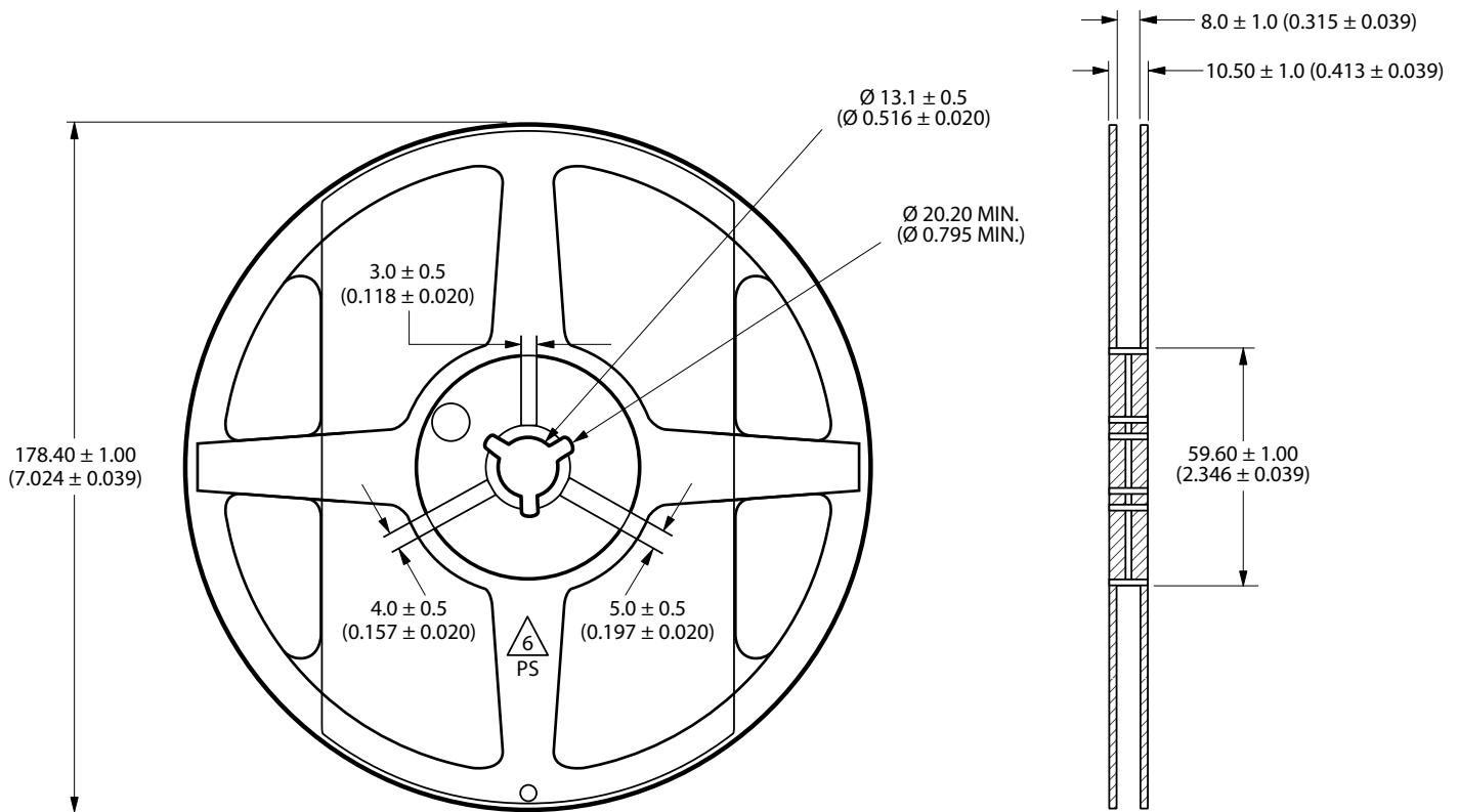
Figure 10: Reel Dimensions
