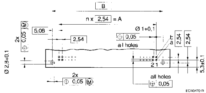
Mounting Holes (component side) for Printed Circuits
