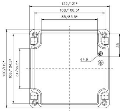
Deckel
