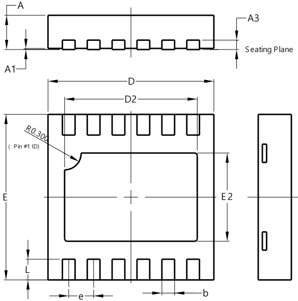
U-DFN3030-12
