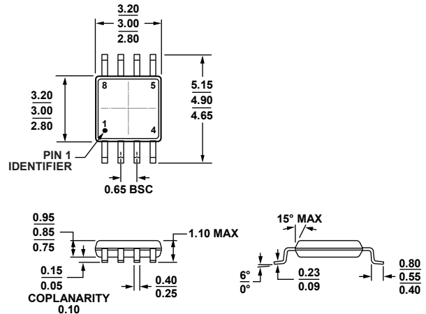
COMPLIANT TO JEDEC STANDARDS MO-187-AA
