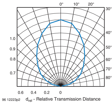
Fig. 4 - Horizontal Directivity
