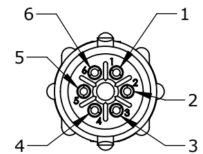
WIRING VIEW W18982-6SG-P-5XX
