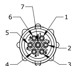
WIRING VIEW W18982-7SG-P-5XX
