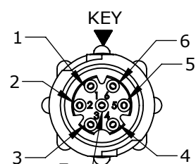
FACE VIEW W18982-7SG-P-5XX 7 POSITION
