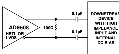
Figure 39. AC-Coupled LVDS or HSTL Output Driver (100 Ω Resistor Can Go on Either Side of Decoupling Capacitors Placed As Close As Possible To The Destination Receiver)
