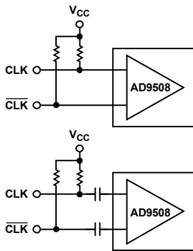
Figure 35. Typical AC-Coupled or DC-Coupled CML Configurations
