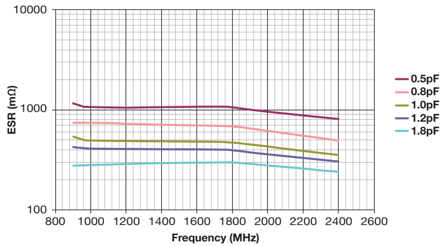
Accu-P® 01005 Typical ESR vs Frequency
