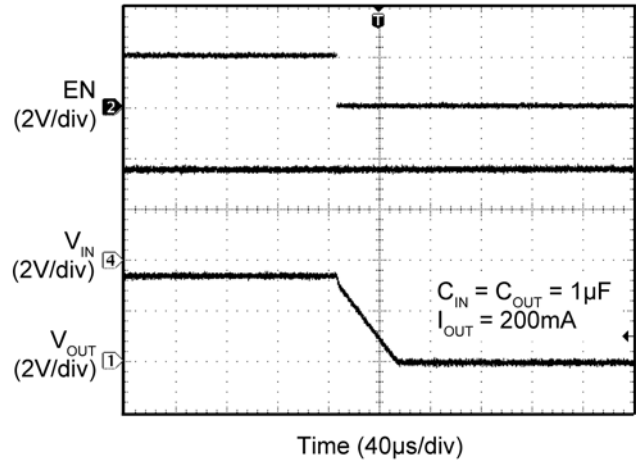
Enable Turn-Off
