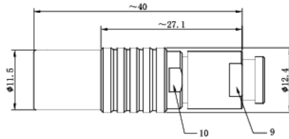
CONNECTOR SOLDER CUP VIEW
