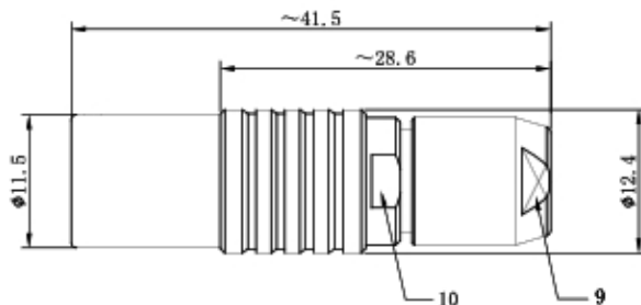
CONNECTOR SOLDER CUP VIEW
