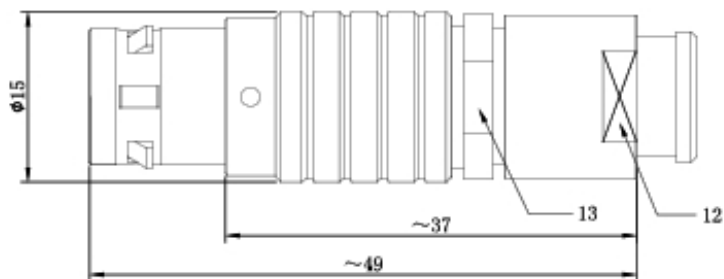
CONNECTOR SOLDER CUP VIEW
