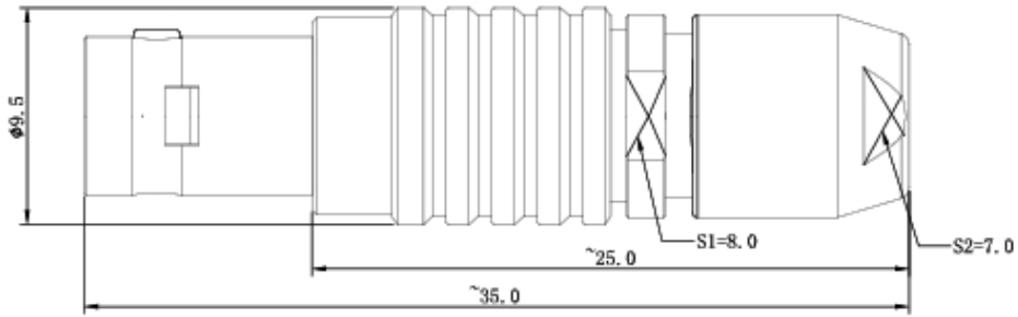
CONNECTOR SOLDER CUP VIEW
