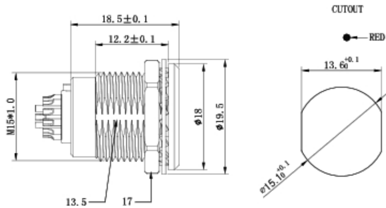
CONNECTOR SIDE VIEW
