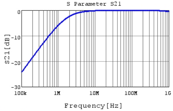
RDER72E102K1K1H03B S21 DCOV, 25degC
