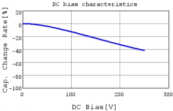
RDER72E102K1K1H03B C-DC bias capchange, 25.0
