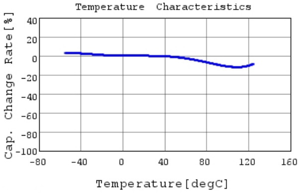
RDER72E102K1K1H03B C-Temp. capchange, DCOV,
