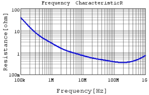
RDER72E102K1K1H03B R DC0V, 25degC
