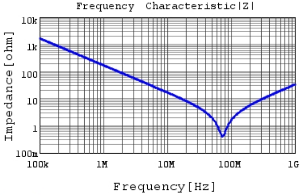
RDER72E102K1K1H03B |Z| DC0V, 25degC
