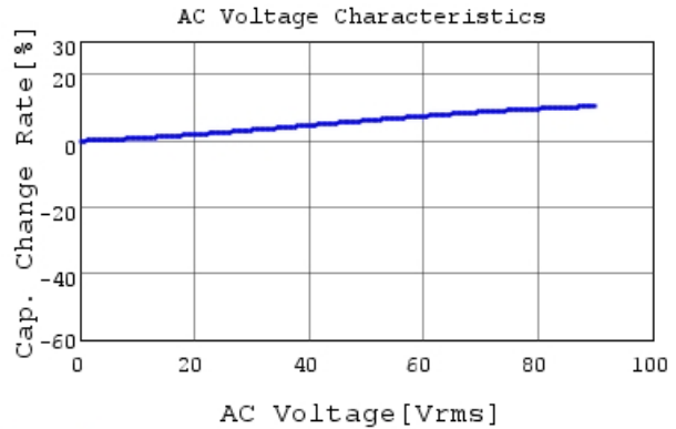
RDER72E102K1K1H03B C-AC Voltage capchange, I
