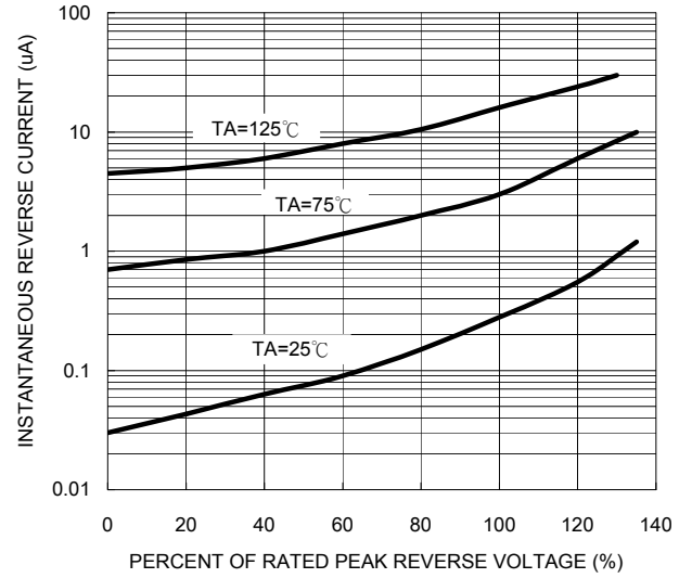
FIG. 2- TYPICAL REVERSE CHARACTERISTICS PER LEG
