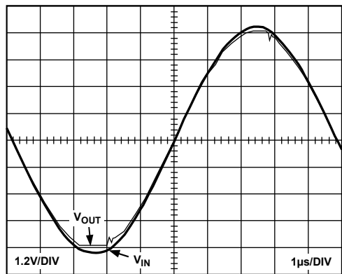
Figure 43. G = +2 Response, V_S = \pm 5\text{V}
