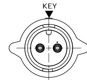
MATING FACE W6382-2SG-P-3XX SHOWN
