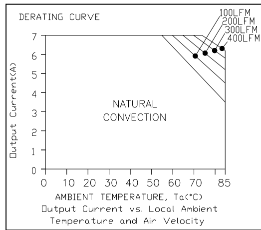
Figure 14. V_{in} = 48 V
