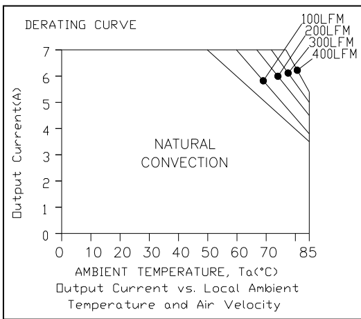
Figure 13. V_{in} = 24 V
