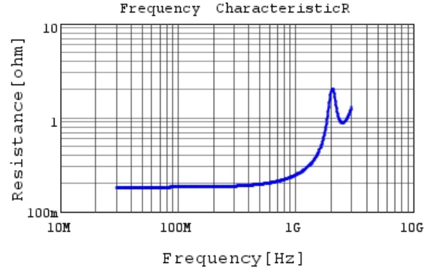
RDE5C1H470J0M1H03A R DCOV, 25degC
