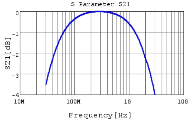
RDE5C1H470J0M1H03A S21 DCOV, 25degC
