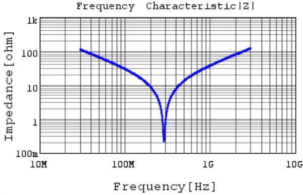
RDE5C1H470J0M1H03A |Z| DCOV, 25degC
