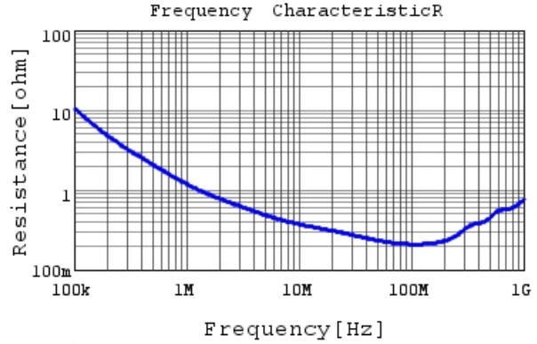
RDER72J222K2M1H03A R DCOV,25degC
