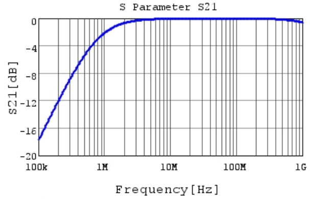
RDER72J222K2M1H03A S21 DCOV, 25degC
