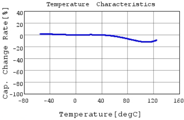
RDER72J222K2M1H03A C-Temp. capchange, DCOV,
