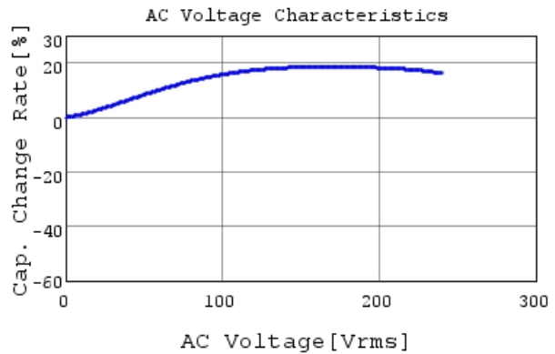
RDER72J222K2M1H03A C-AC Voltage capchange, I
