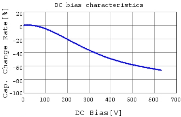
RDER72J222K2M1H03A C-DC bias capchange, 25.0
