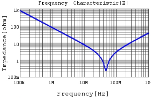
RDER72J222K2M1H03A |Z| DCOV,25degC
