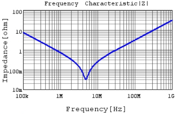
RDER71H224K1P1H03B |Z| DCOV, 25degC
