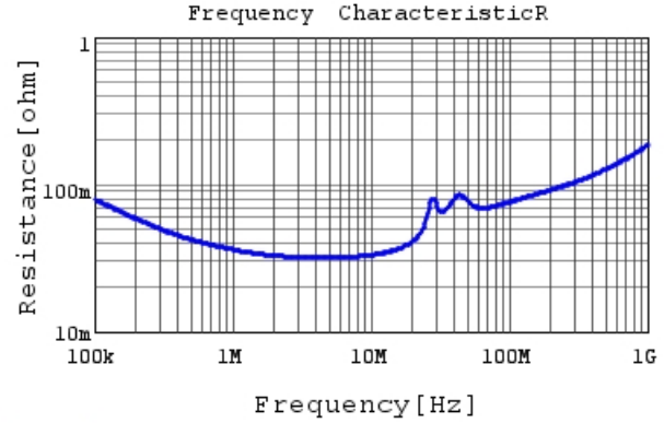
RDER71H224K1P1H03B R DCOV, 25degC
