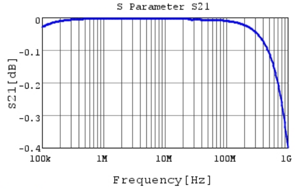
RDER71H224K1P1H03B S21 DC0V, 25degC
