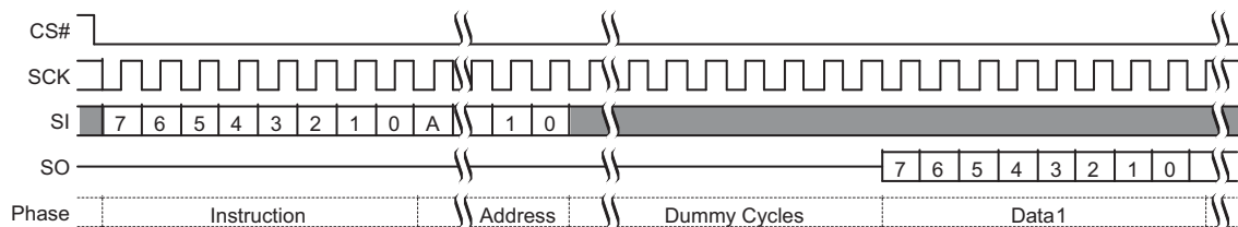
Figure 73. Read Any Register Read Command Sequence [50]
