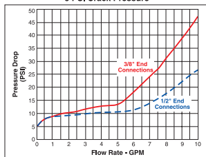
CB6 Check Valve Flow Rate vs. Pressure Drop CB-Series Check Valve – Size CB6 5 PSI Crack Pressure
