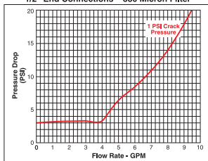
CBF8 Filter Check Valve Flow Rate vs. Pressure Drop CB-Series Check Valve – Size CBF8 1/2" End Connections – 380 Micron Filter
