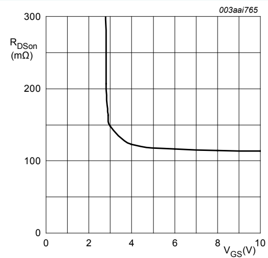
Fig. 7. Drain-source on-state resistance as a function of gate-source voltage; typical values T_j = 25\text{ °C}; I_D = 2\text{ A}
