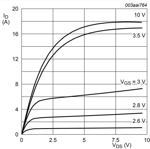
Fig. 6. Output characteristics; drain current as a function of drain-source voltage; typical values T_j = 25\text{ °C}; t_p = 300\text{ }\mu\text{s}
