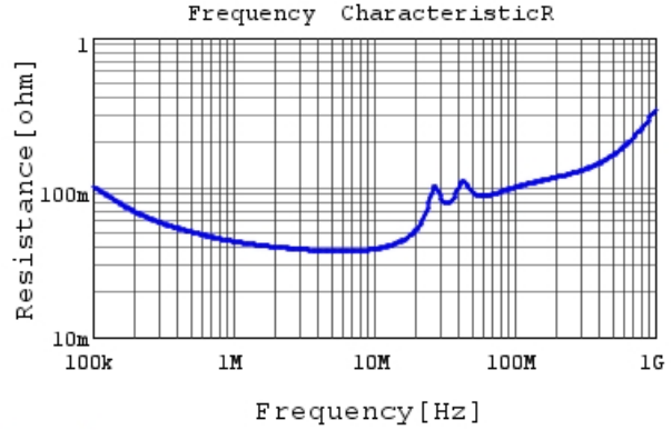
RDER72E224K3M1H03A R DCOV, 25degC
