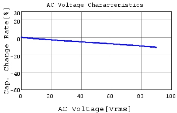
RDER72E224K3M1H03A C-AC Voltage capchange, I
