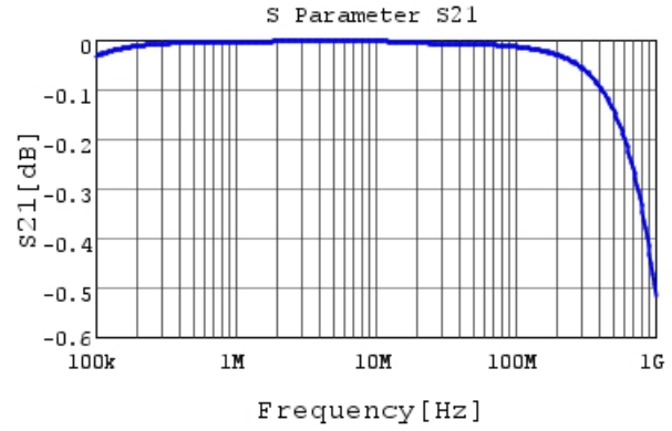
RDER72E224K3M1H03A S21 DCOV, 25degC
