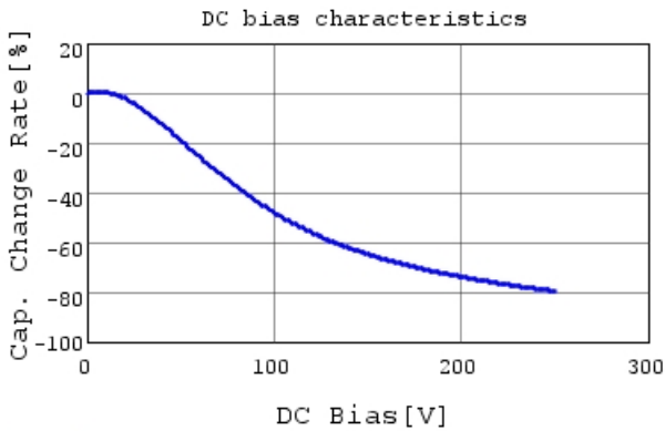
RDER72E224K3M1H03A C-DC bias capchange, 25.0
