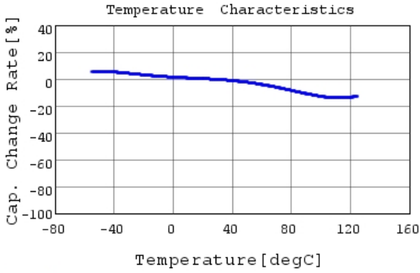
RDER72E224K3M1H03A C-Temp. capchange, DCOV,
