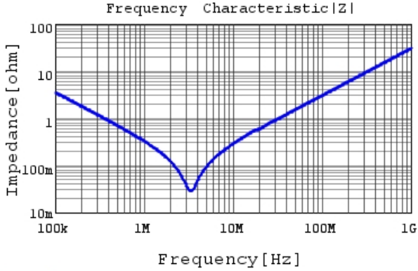
RDER72A474K1S1H03A |Z| DCOV, 25degC
