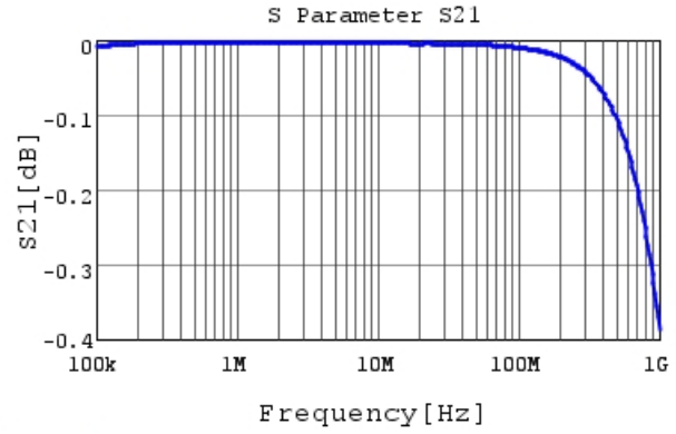
■ RDER72A474K1S1H03A S21 DC0V, 25degC
