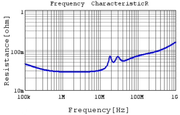
RDER72A474K1S1H03A R DCOV, 25degC
