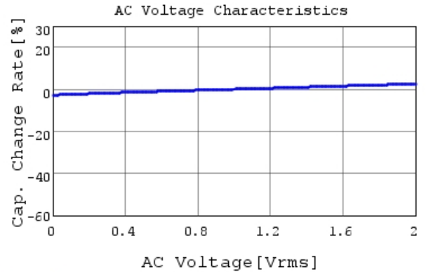
RDER71H224K1S1H03A C-AC Voltage capchange, I
