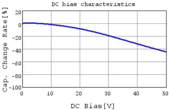
RDER71H224K1S1H03A C-DC bias capchange, 25.0
