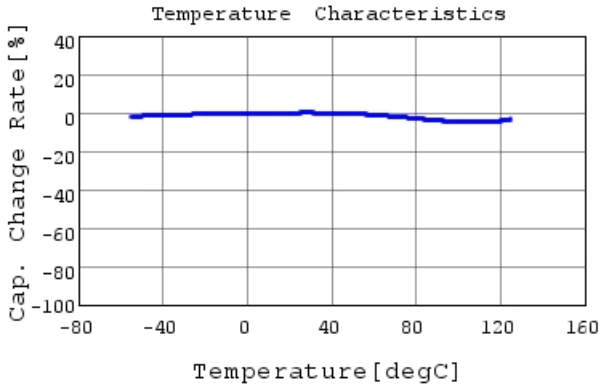
RDER71H224K1S1H03A C-Temp. capchange, DC0.0V
