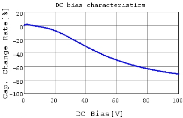
RDER72A104K1P1H03B C-DC bias capchange, 25.0
