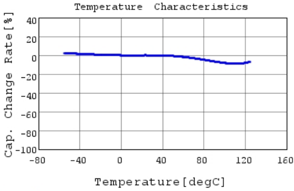
RDER72A104K1P1H03B C-Temp. capchange, DC0.0V
