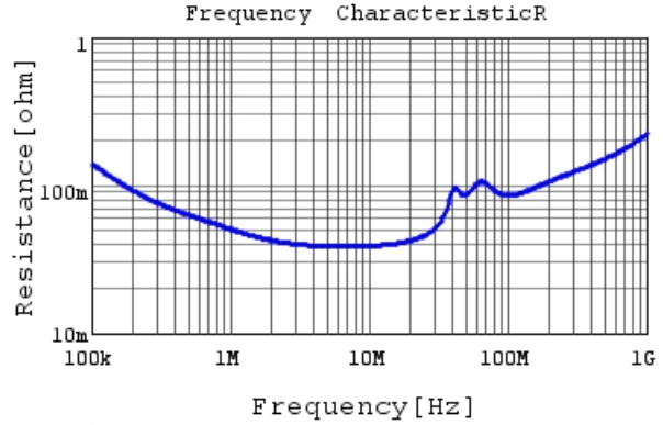
RDER72A104K1P1H03B R DCOV, 25degC
