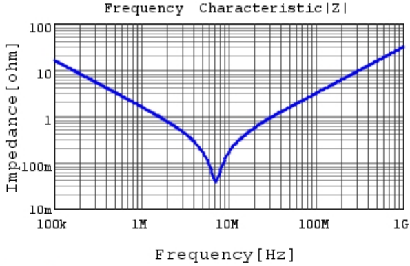
RDER72A104K1P1H03B |Z| DCOV, 25degC
