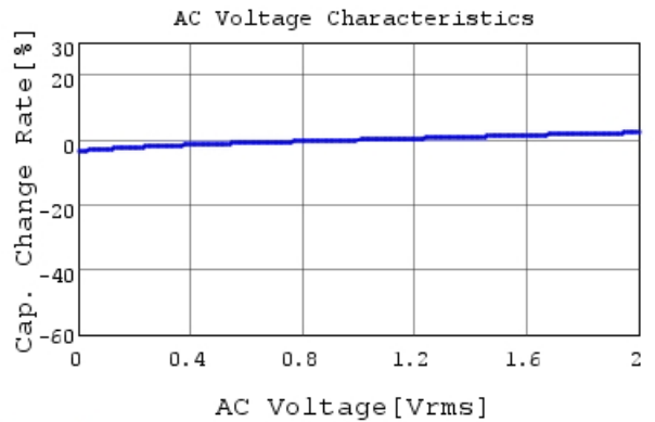
RDER72A104K1P1H03B C-AC Voltage capchange, I
