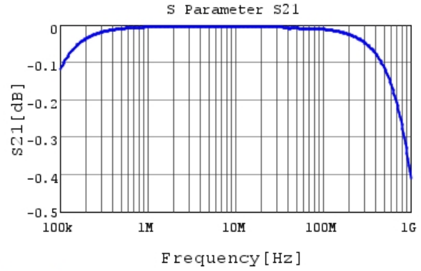
RDER72A104K1P1H03B S21 DC0V, 25degC
