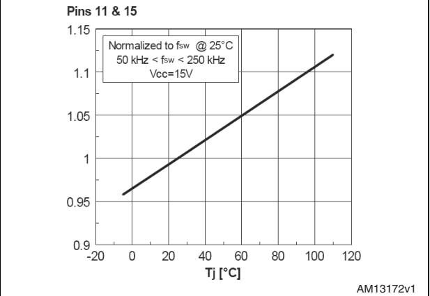
Figure 10. Oscillator ramp vs. junction temperature
