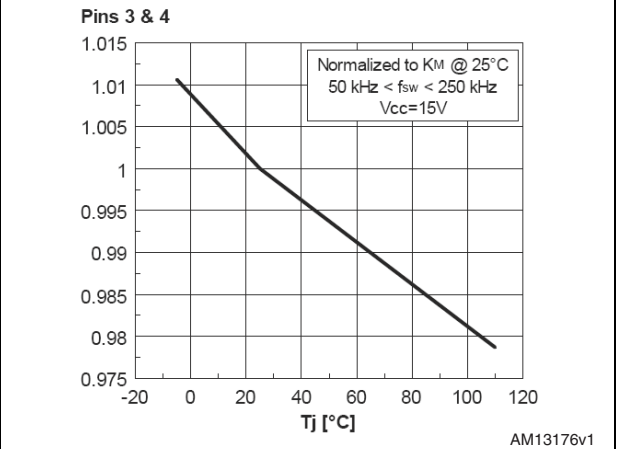
Figure 12. Current mirroring ratio vs. junction temperature
