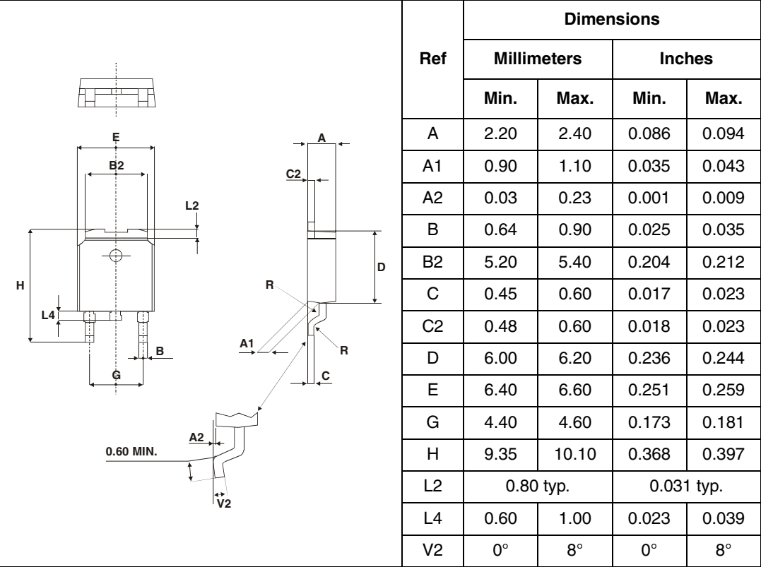
Figure 11. DPAK dimensions
