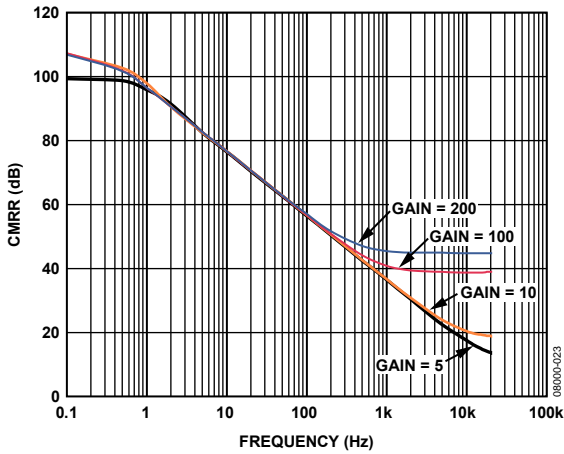
Figure 12. CMRR vs. Frequency, RTI
