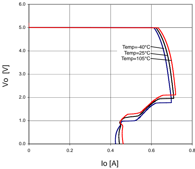
Figure 29. OCP
