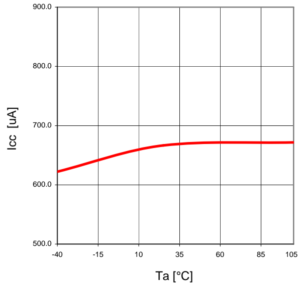
Figure 22. Ta-Icc
