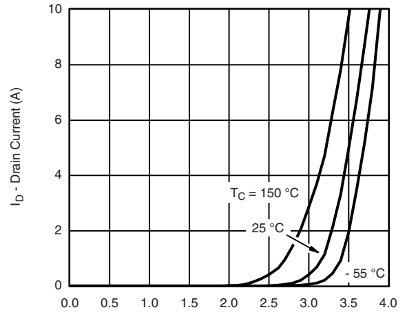
T_C = 150\text{ °C} 25\text{ °C} -55\text{ °C} Transfer Characteristics
