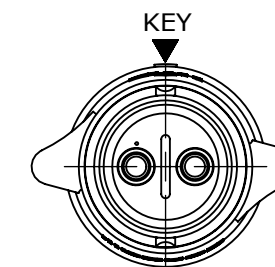
WIRING END ASSY: W6380-2SG-P-5XX SHOWN WITHOUT HARDWARE
