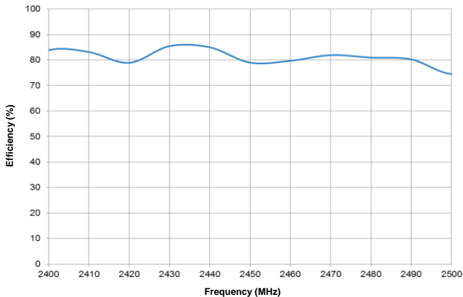
2.4 GHz Efficiency
