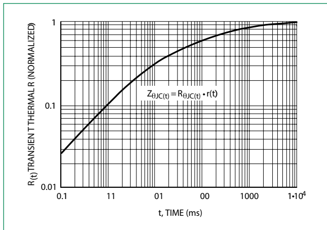
Figure 3. Transient Thermal Response
