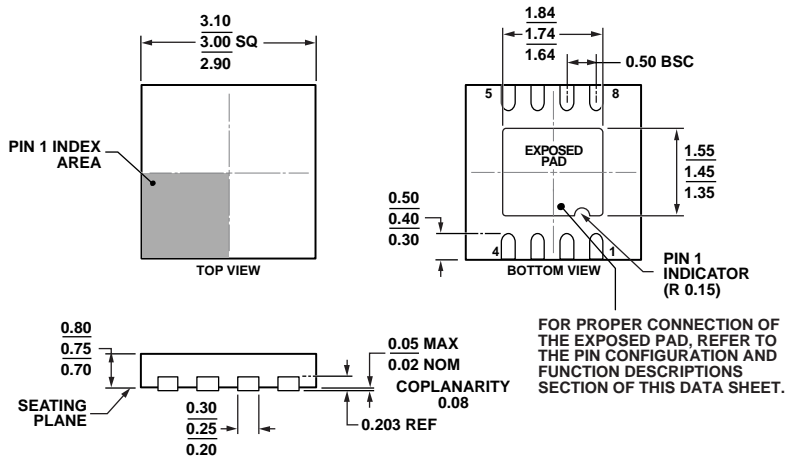
COMPLIANT TO JEDEC STANDARDS MO-229-WEED Figure 73. 8-Lead Lead Frame Chip Scale Package [LFCSP_WD] 3 mm x 3 mm Body, Very Very Thin, Dual Lead (CP-8-13) Dimensions shown in millimeters
