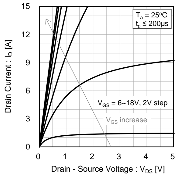
Fig.5 T_a = 25^\circ\text{C} Typical Output Characteristics(II)
