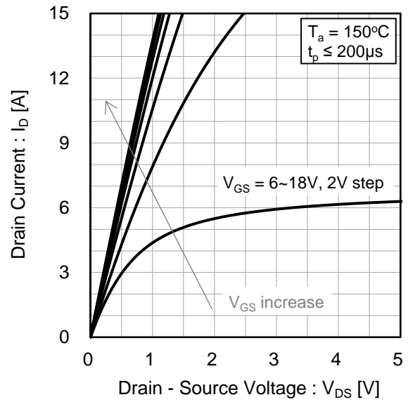
Fig.8 T_a = 150^\circ\text{C} Typical Output Characteristics(II)
