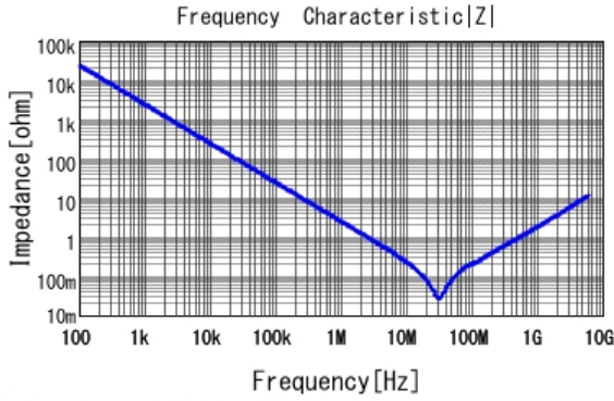
GCM155R71C683KA55 |Z| DCOV, 25degC
