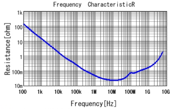
GCM155R71C683KA55 R DCOV, 25degC
