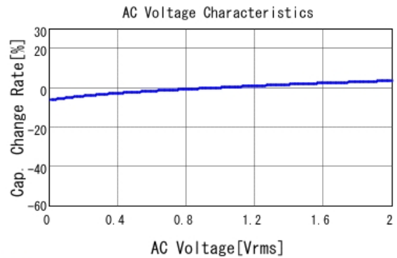
GCM155R71C683KA55 C-AC Voltage capchange, DCOV, 25.0d
